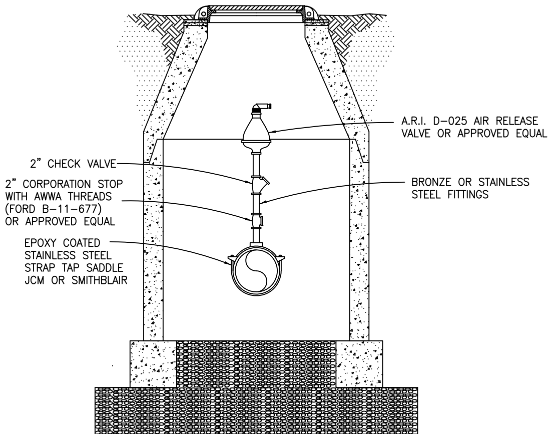
SECTION "Y-Y"
