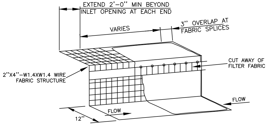
ISOMETRIC
