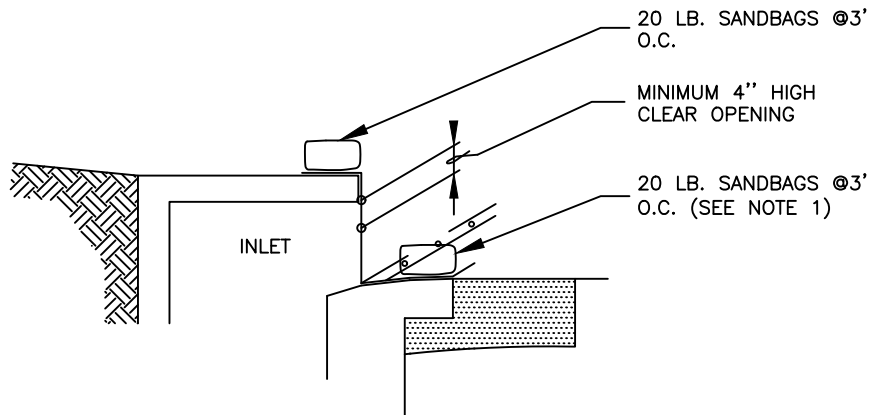
CROSS SECTION
